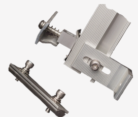
MIBET 3-PANEL ROOF- MOUNTING KIT (ALL MATERIALS INCLUDED) K572.00/KIT
